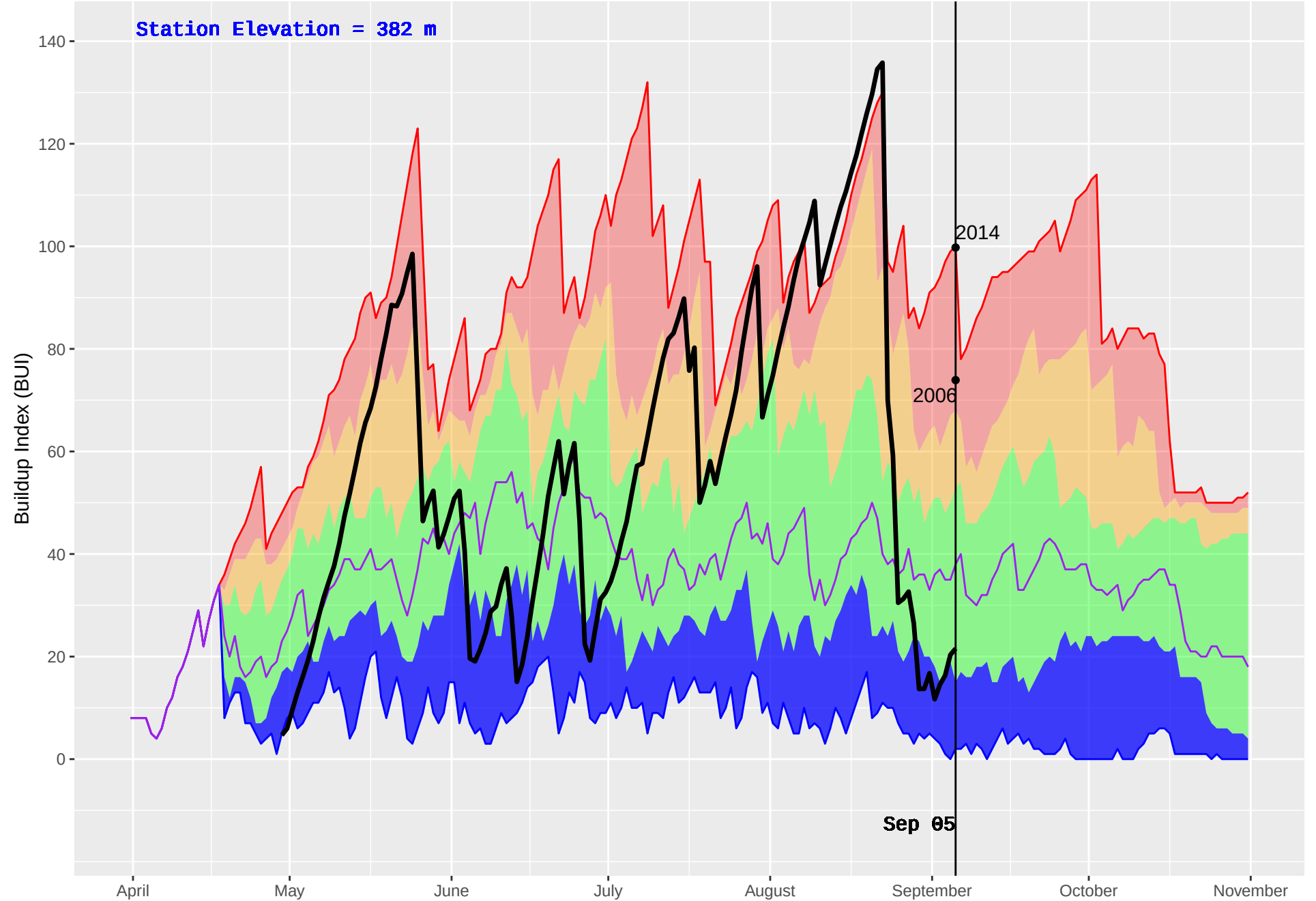
FORT NELSON FS (599) : Historical (1999–2016) and Current (2018) Daily Buildup Index (BUI)
